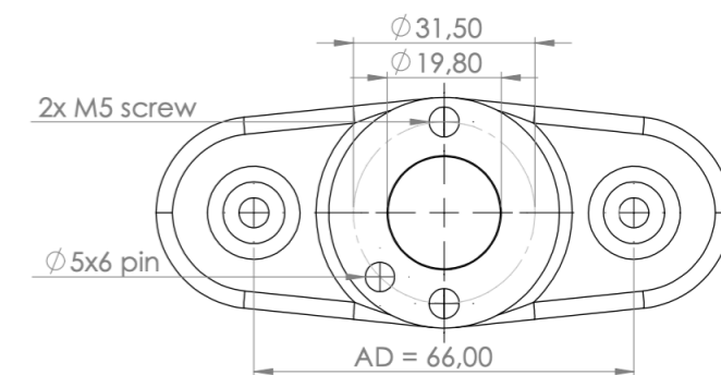
Connector ISO 9404-1-31.5-2-M5
