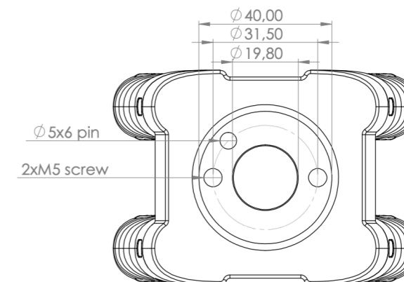
Connector ISO 9404-1-31.5-2-M5
