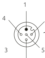
Muting sensors 1 - 2 (blu) M12 5-pole - Female
