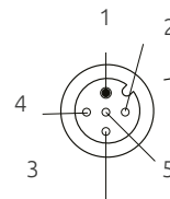
Muting sensors 3 - 4 (red) M12 5-pole - Female
