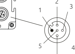
Muting sensors 1 - 2 (blu) M12 5-pole - Female
